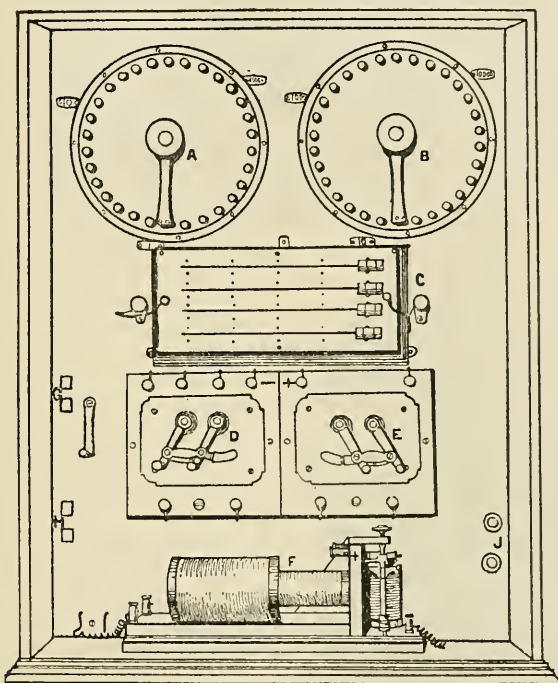
FIG. 113. — Regulator switch board for continuous and induced currents.
